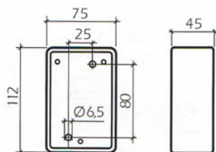
Enclosure
