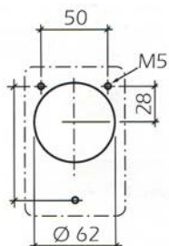
Mounting Holes
